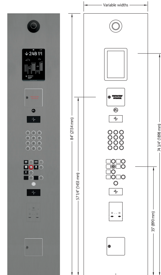
Swing Car Operating Panel for KONE 24/7 Emergency Video Communications
