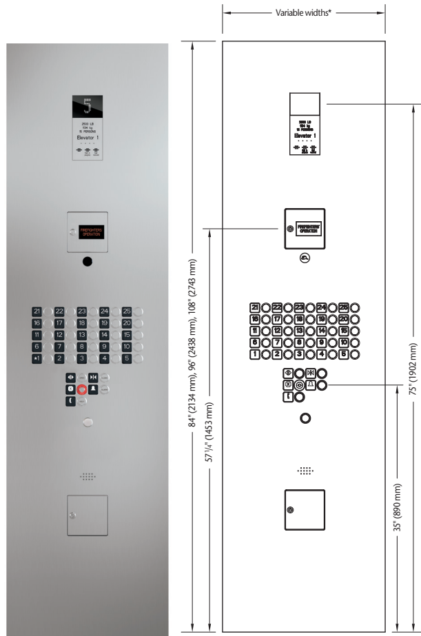
Swing Car Operating Panel
