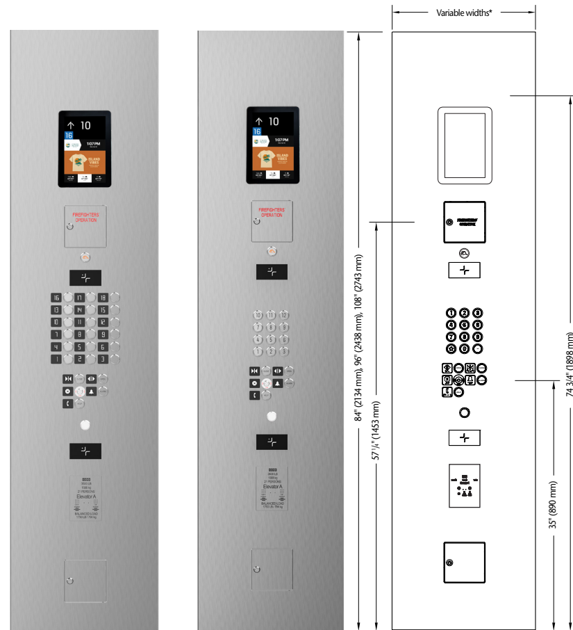
Swing Keypad Car Operating Panel with KONE Infotainment†
