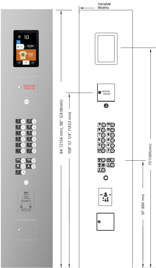
Swing Car Operating Panel with KONE Infotainment*
