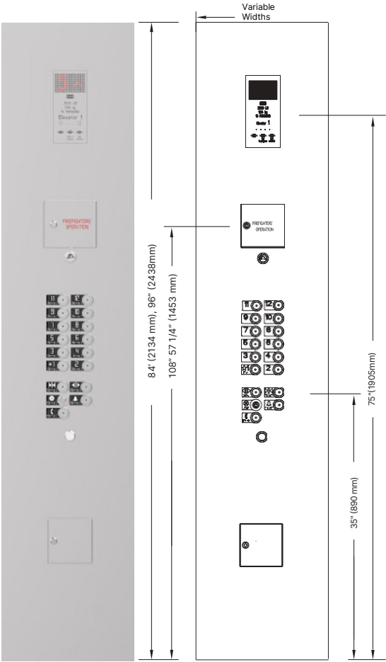
Swing Car Operating Panel* Stainless Steel
