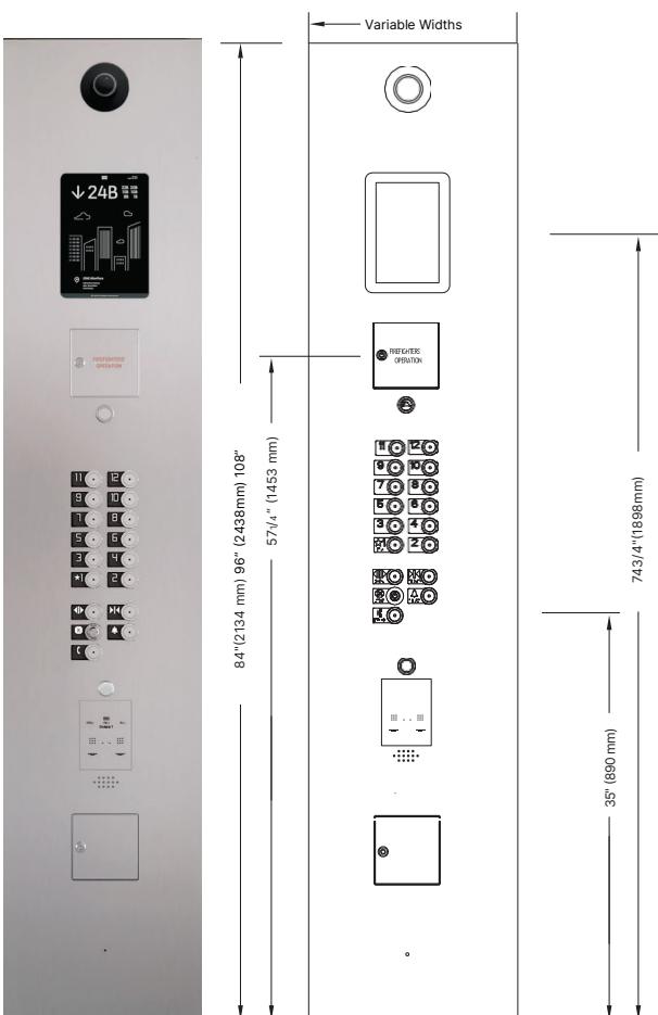
Swing Car Operating Panel For KONE 24/7 Emergency Video Communications
